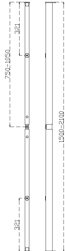
MBR 16-22 * 1600-2200 mm
